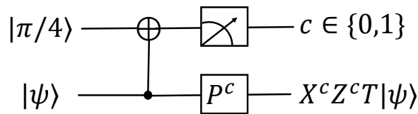
Figure 10.1: Teleporting into a T gate. The state |\pi/4\rangle is defined in (10.1).
