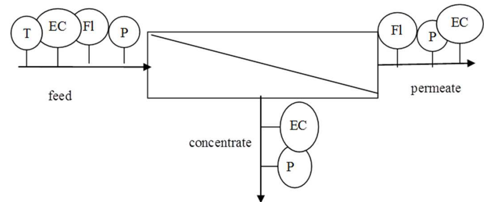
Figure 9: monitoring equipment for the test rig
