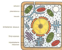
Fig. 738 The cell and its membranes e
