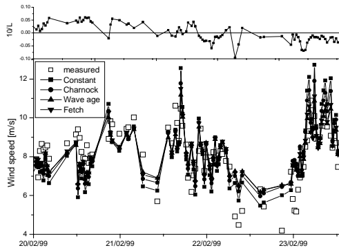
Figure 5: Time series plot of atmospheric stability (expressed as 10/L with L = Monin-Obukhov length) and measured and modelled neutral wind speeds at 10 m height
